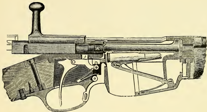
The Berthier Rifle.
